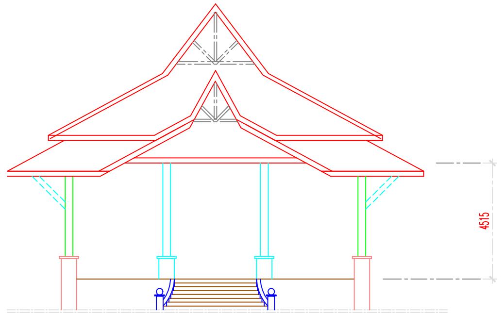
PANDANGAN HADAPAN
