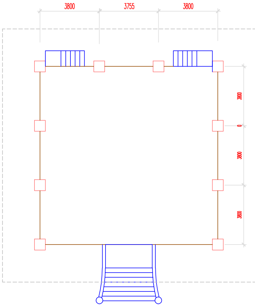
PLAN LANTAI WAKAF LANAI MATIC
